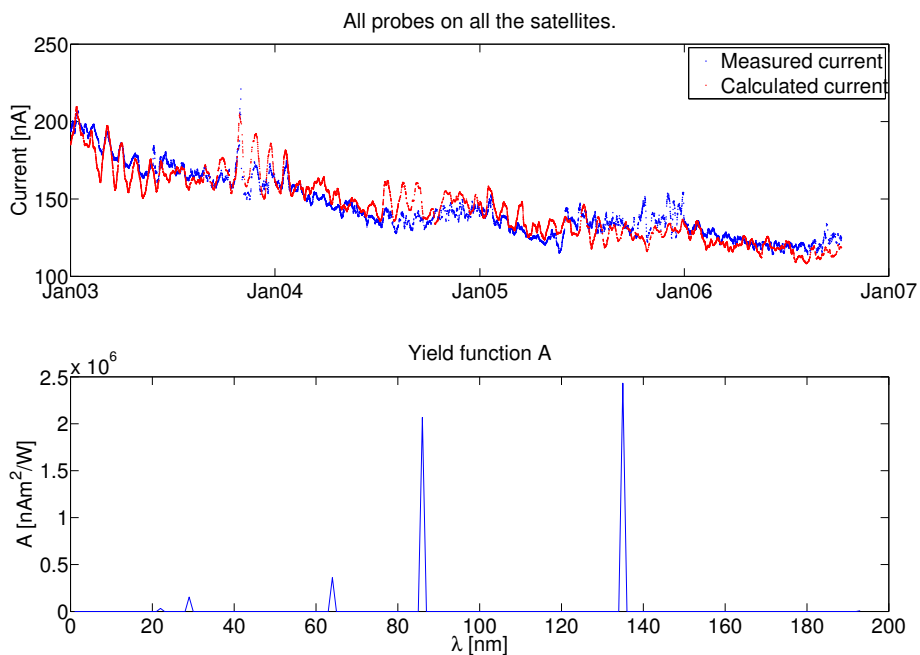
Figure 5.6: The calculated photoelectron current from the calculated yield function shown below. The measured photoelectron current is the blue on in the top plot
