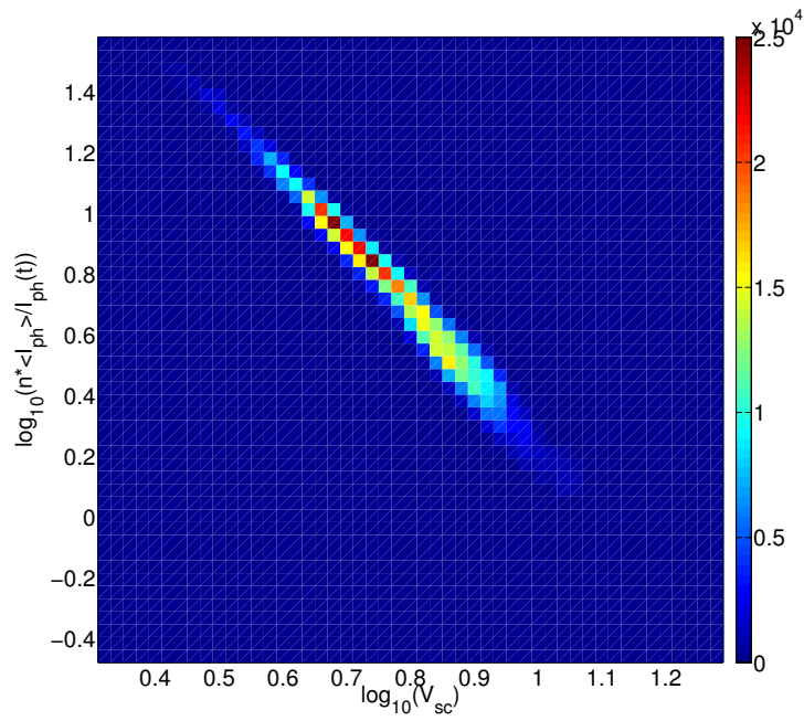
Figure 6.4: \text{Log}_{10}(\frac{n \langle I_{ph} \rangle}{I_{ph}}) versus \text{Log}_{10}(V_{sc}) . The photoelectron current is used as a EUV proxy
