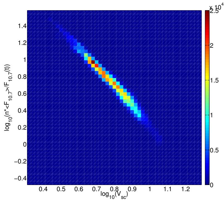
Figure 6.3: \text{Log}_{10}(\frac{n \langle F_{10.7} \rangle}{F_{10.7}}) versus \text{Log}_{10}(V_{sc}) . Normalized with the EUV proxy F_{10.7} .
