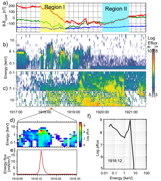
Figure 2. DMSP F14 observations. a) Magnetic field with IGRF model subtracted. Components are approximately: red eastward, green poleward, blue upward. b,c) electron and ion spectrograms. 30 s of data around the auroral arc, d) electron spectra and e) electron energy flux projected to ionosphere. f) electron number flux spectra from inside the inverted-V event.
