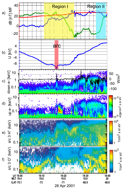
Figure 3. Overview plot of s/c 3 data. a) Magnetic field disturbance dB, subtracting the Tsyganeko 89 model, in field aligned coordinates. The approximate directions are — green eastward, blue poleward, red field-aligned. b) Potential integrating E along the satellite orbit. To obtain full E from EFW spin plane measurements we assume that E_{\parallel} = 0 . c,d) Spectrograms of electrons propagating parallel and antiparallel to B. c) line plot shows integrated electron energy flux, labels are on the right side. e,f) \text{H}^+ and \text{O}^+ spectrograms integrated over all pitch angles.
