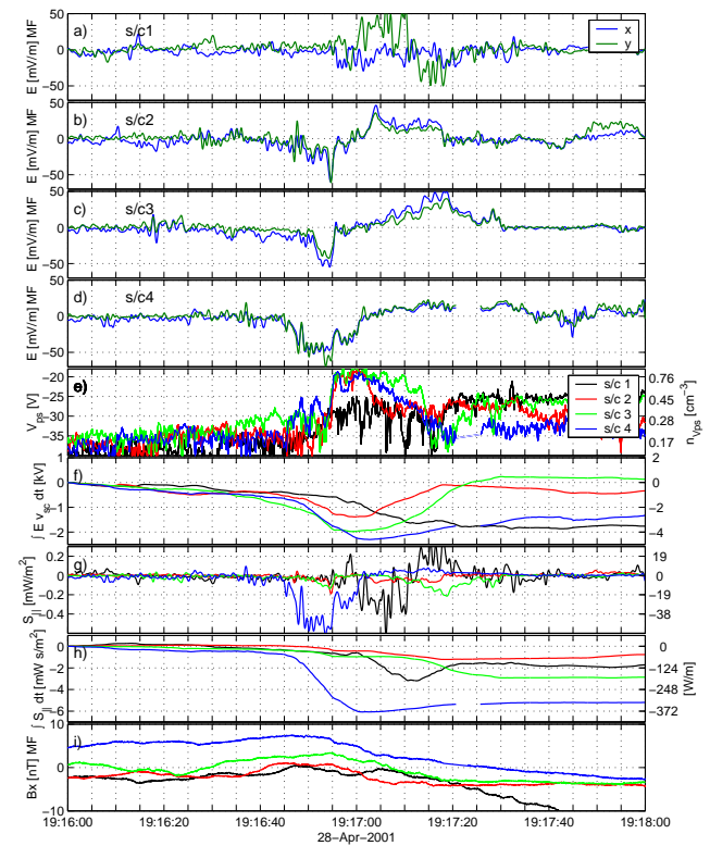
Figure 4. 2 min overview plot from all four s/c. The data have been low-pass filtered at 1 Hz. a–d) E in mean field coordinates, x is poleward and y is eastward. e) Probe to spacecraft potential and derived density estimate. f) integrated potential, the labels on the right show values if the arc motion is taken into account. g) Field-aligned Poynting flux calculated from total E and dB. h) integrated Poynting flux. For g) and h) labels on the right show values at the ionosphere. i) Poleward component of dB in field aligned coordinates.
